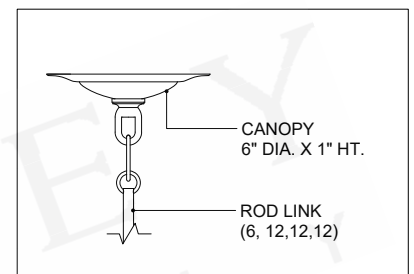
CANOPY DETAIL
