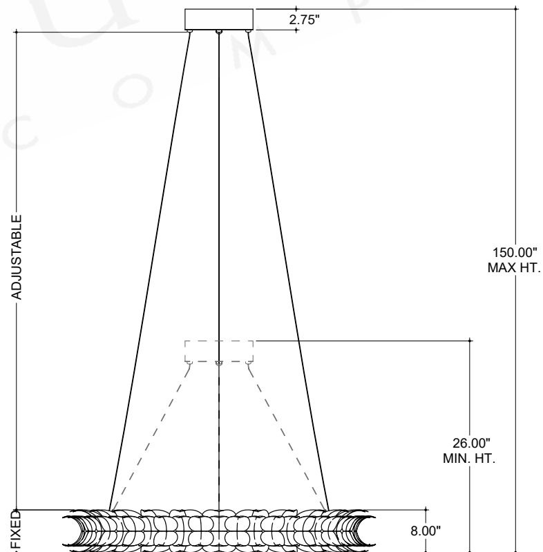
FRONT VIEW
