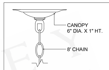
CANOPY DETAIL
