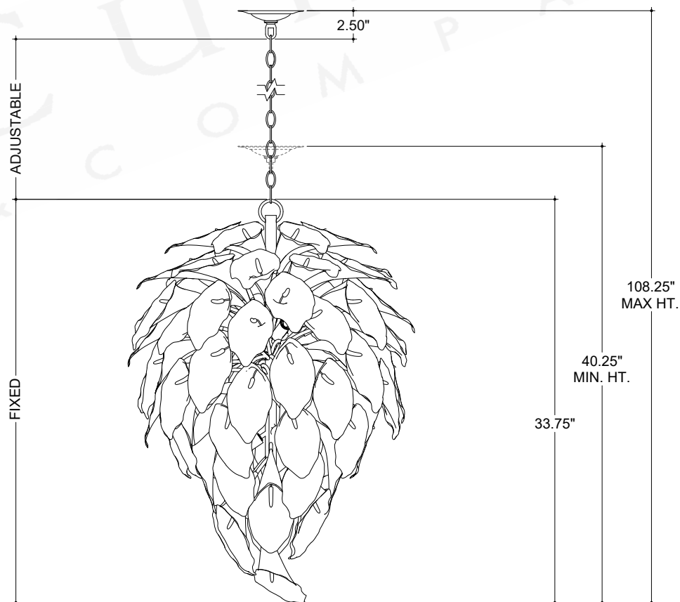
FRONT VIEW
